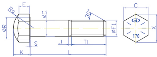
TRACK BOLT
