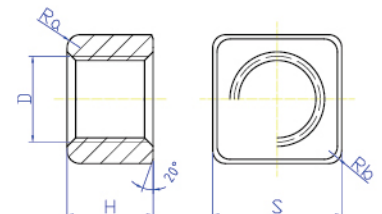
SQUARE TRACK NUT
