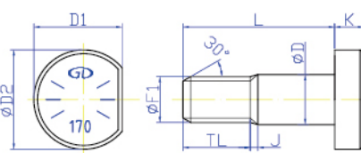
"D" HEAD SEGMENT BOLT
