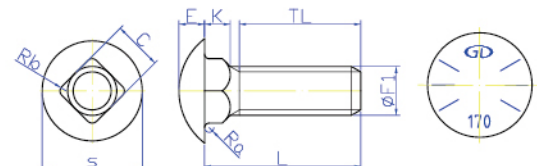
CARRIAGE BOLT
