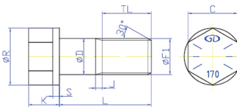
FLAT HEAD TRACK BOLT WASHERED
