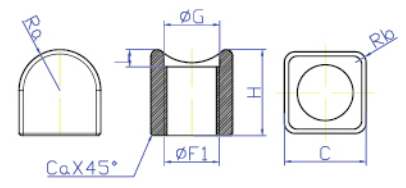
SPHERE SQUARE TRACK NUT
