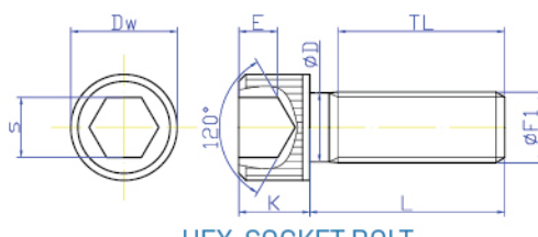
HEX. SOCKET BOLT
