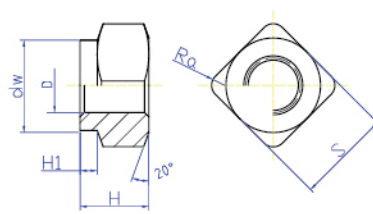
SQUARE COLLAR TRACK NUT
