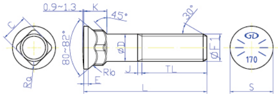
PLOW BOLT
