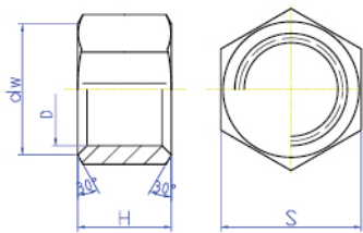
PLOW HEX. NUT & HEX. SEGMENT NUT
