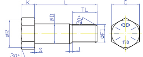
HEX. HEAD BOLT / SEGMENT BOLT
