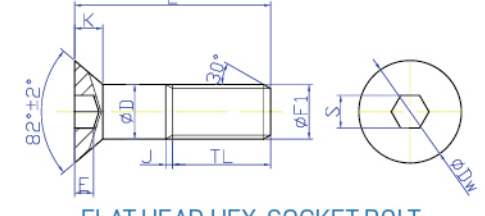
FLAT HEAD HEX. SOCKET BOLT
