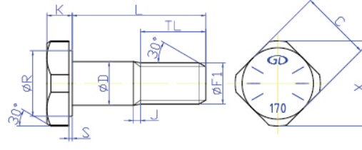
SQUARE HEAD SEGMENT BOLT
